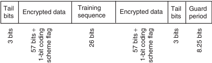
Figure 6.5 Physical structure of a GPRS burst.
