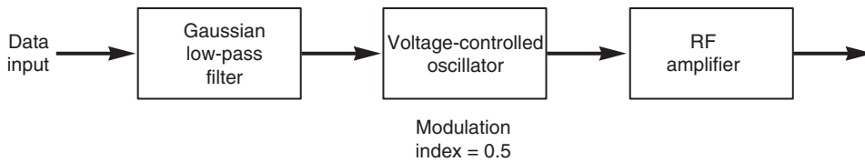
Figure 3.18 Generating GMSK using a Gaussian filter and a frequency modulator with the modulation index set to 0.5.
