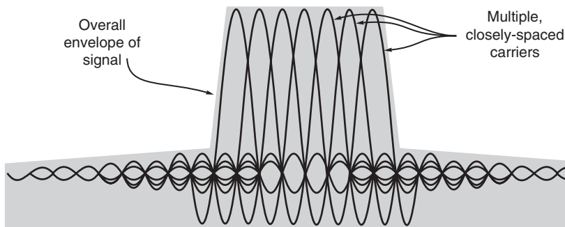
Figure 3.24 The spectrum of a COFDM signal.
