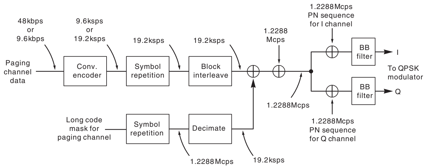
Figure 8.4 Paging channel generation.
