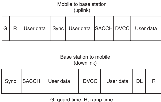
Figure 7.1 Logical channels or fields within the Data Traffic Channel.
