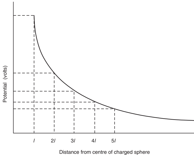
Figure 2.2 Variation of potential with distance from the charged sphere.
