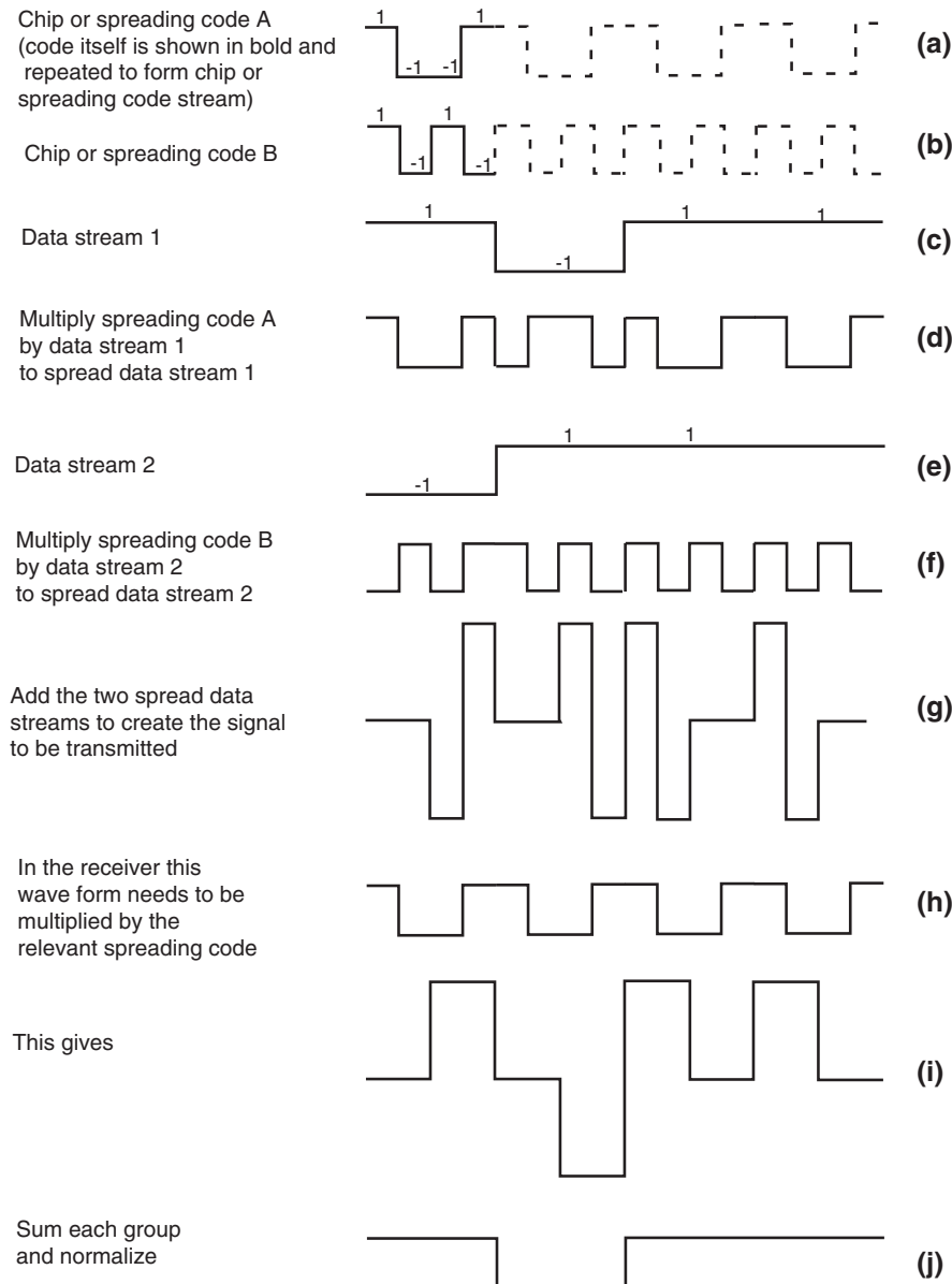
Figure 3.22 Operation of direct sequence spread spectrum coding and decoding.
