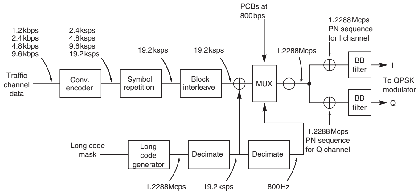
Figure 8.8 Forward channel generation.
