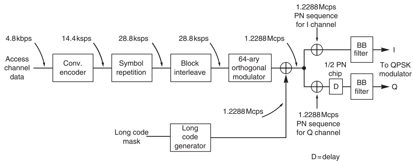
Figure 8.10 Reverse access channel generation.
