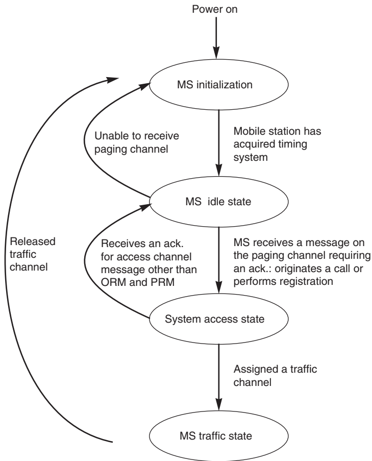
Figure 8.11 Basic four states of call processing.
