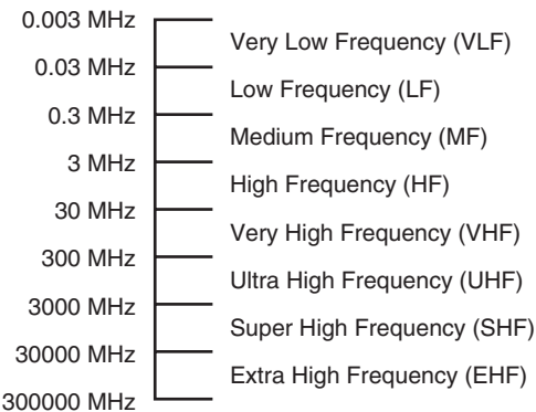
Figure 2.6 The electromagnetic wave spectrum.
