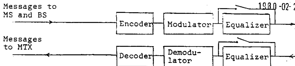
Fig. 4.6.1 Functional block diagram of the 1200 Baud signaling equipment at MTX
