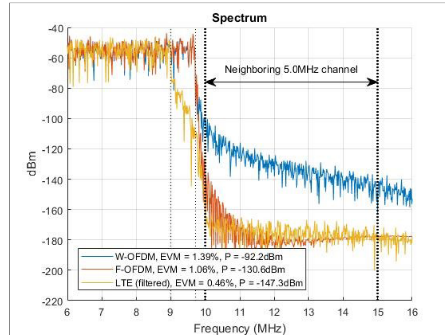
Spectrum measurements for LTE and candidate 5G modulation techniques: CP-OFDM with ACLR filtering (100 RBs, used in LTE), W-OFDM (108 RBs), and F-OFDM (108 RBs).
