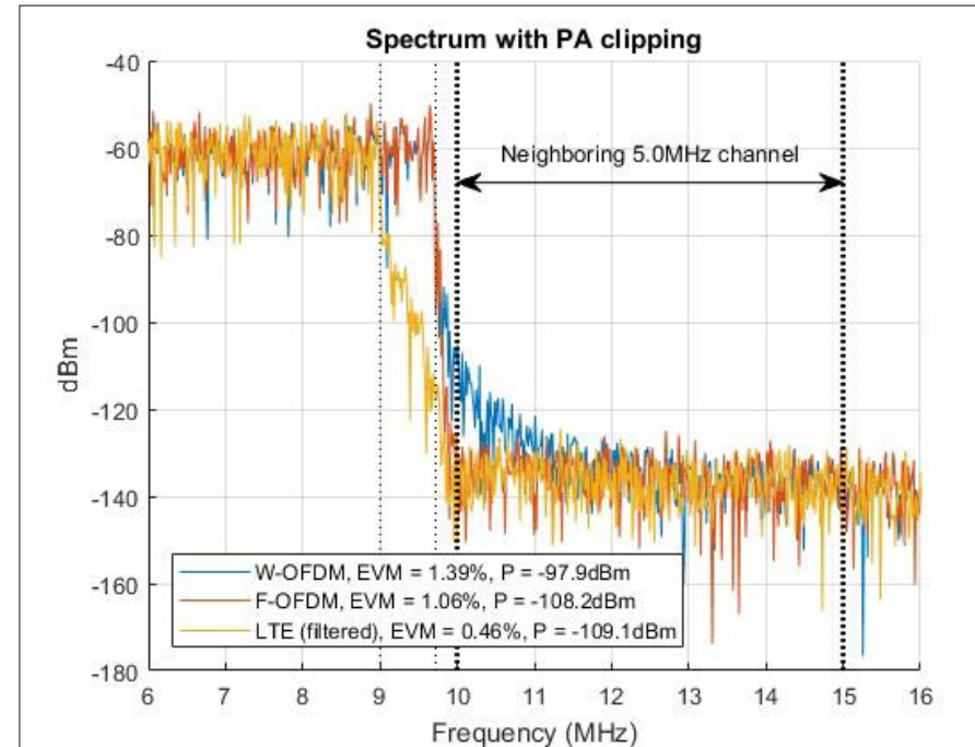
Spectrum of CP-OFDM, W-OFDM (108RBs), and F-OFDM (108RBs) with nonlinear power amplifier (PA).
