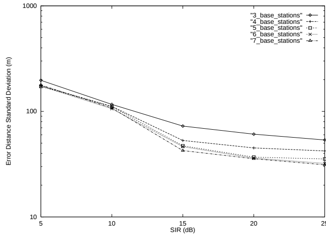
Figure 7: Radial Error Distance Standard Deviation (Rising Edge Detection, 4 Ray Channel)
