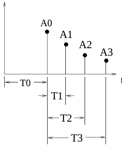
Figure 5: Four Ray Channel Impulse Response
