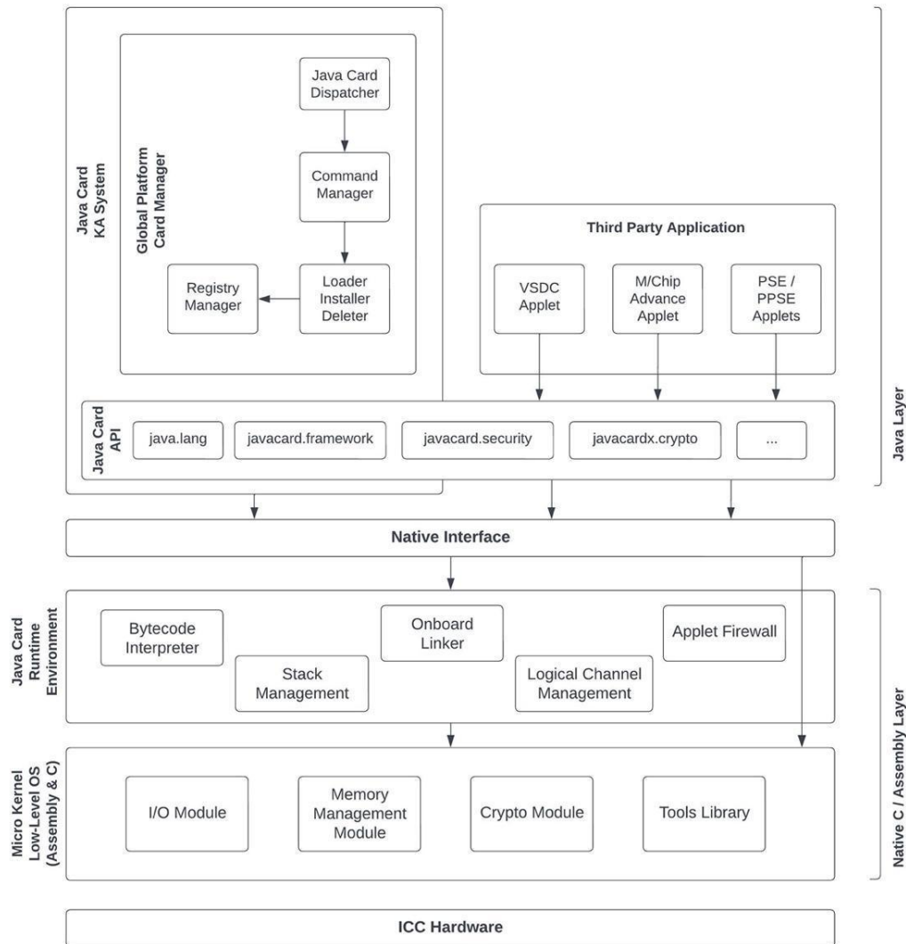
Fig. 1. Java card operating system high-level architecture.
