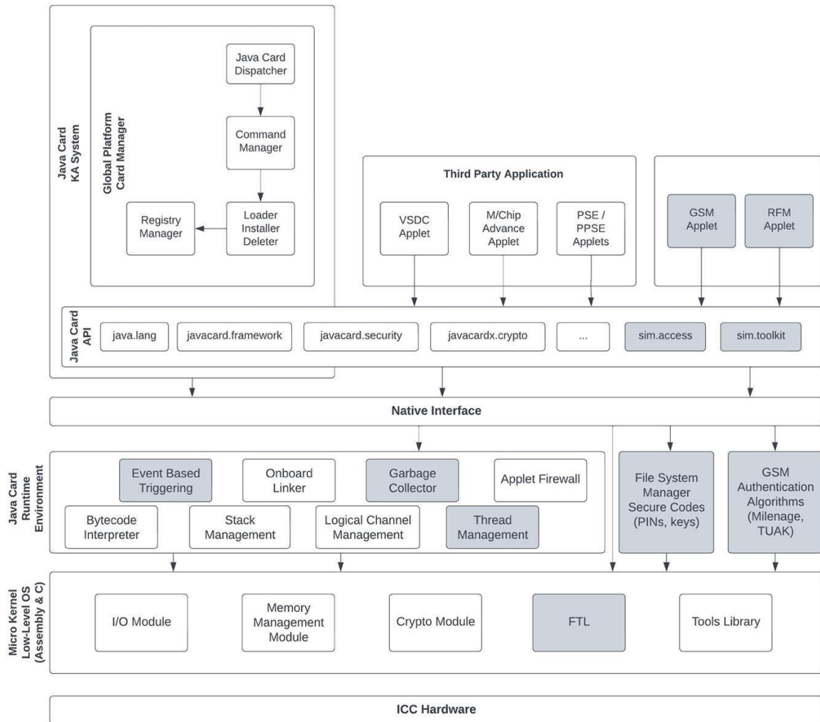
Fig. 4. High-end architecture of the proposed Java Card based SIM operating system
